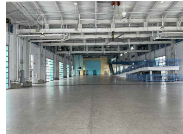
WEST BAGGAGE AREA (LOOKING EAST)
